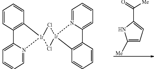
iridium chloro-bridged dimer B
