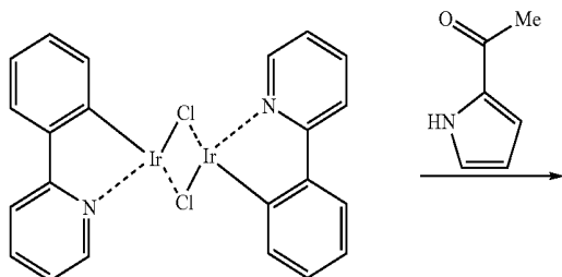
iridium chloro-bridged dimer B
